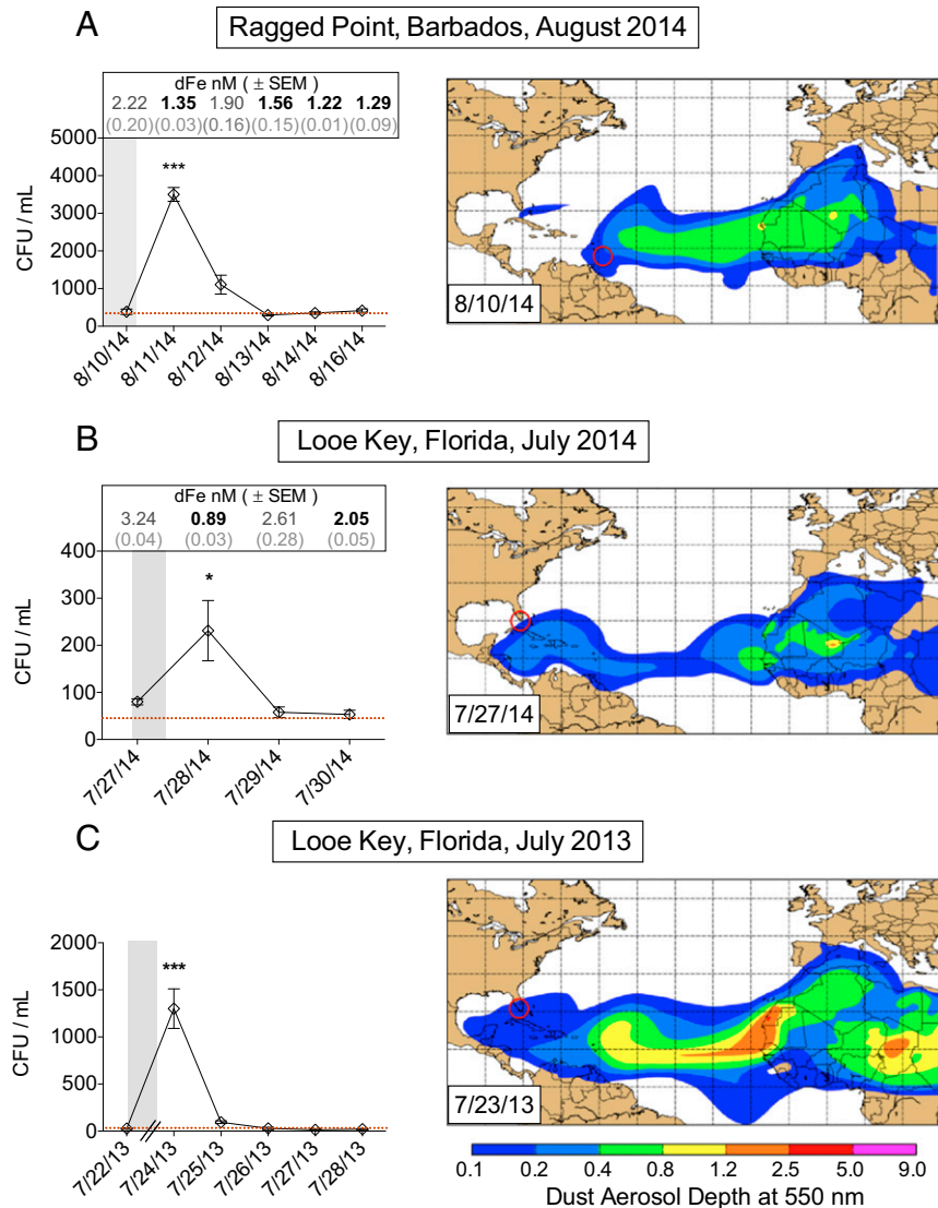
Fig. 4. Vibrio response to natural SDEs. (Left) Vibrio concentrations (cfu·mL -1 ) ( n = 3 ; mean \pm SEM) in surface waters during the arrival (shaded bar) of SDE and 3–5 d after dust arrival in Barbados (A) and the Florida Keys (B and C). Dashed lines represent baseline surface water Vibrio concentrations ( 348 \pm 122 SEM, n = 3 for Barbados and 45.4 \pm 2.5 SEM, n = 42 for Florida), determined during the dust season (April– August) but not associated with a SDE. For each SDE, Vibrio concentration on the date of peak response was significantly different from all other dates. * P < 0.05 ; *** P < 0.001 . Double hash indicates non-consecutive sampling date (C). Mean ( \pm SEM, n = 3 ) dFe concentrations were determined for A and B only; bold values indicate significantly lower dFe than that observed on the dust arrival date (ANOVA P < 0.05 ). (Right) Modeled dust aerosol depths (Naval Research Laboratory ( www.nrlmry.navy.mil/aerosol/ ) (study site indicated by red circle).
