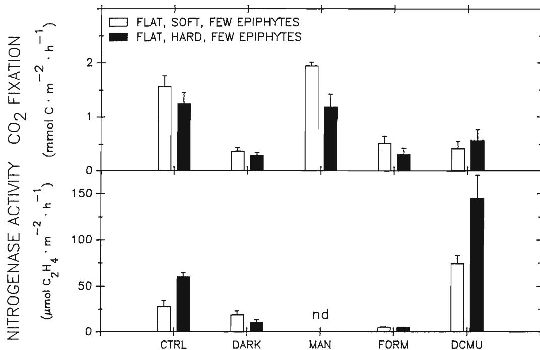
Fig. 8. Results of the addition of inhibitors and DOC on CO 2 and N 2 fixation by soft and hard mats with few epiphytes. Abbreviations are CTRL (control), DARK (dark incubation), MAN (mannitol DOC), and FORM (formalin). Values are the mean \pm 1 SD.
