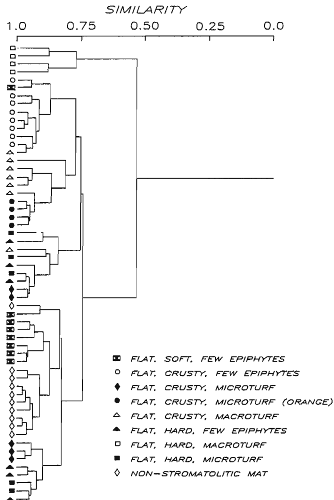
Fig. 3. Cluster analysis dendrogram based on the similarity of “photopigment profiles” for nine different mat types. Flat, crusty, microturf (orange) refers to a particular type of flat, crusty, microturf mat that had a distinctive orange coloration. Symbols that are clustered together in the dendrogram indicate that the photopigments for a particular mat type were more similar to one another than to different mat types.
