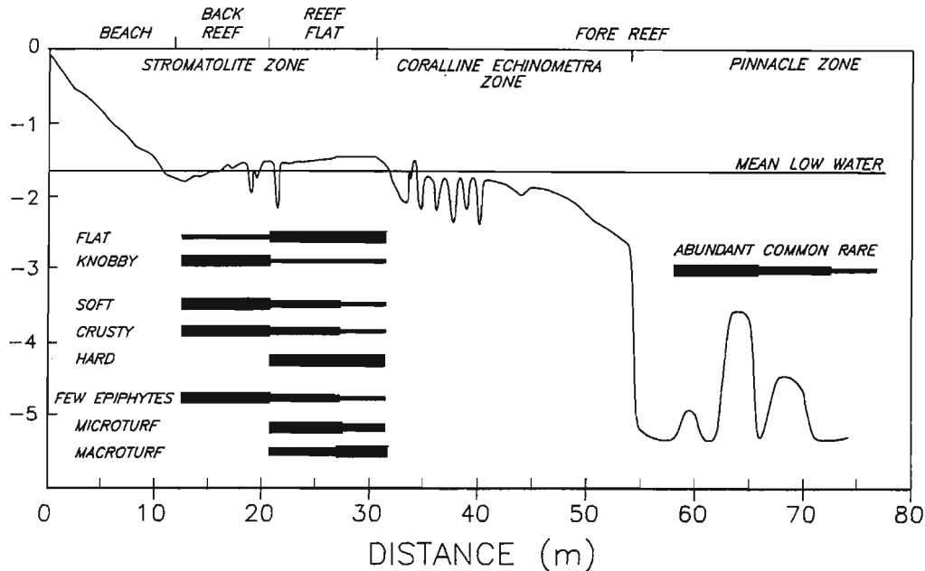
Fig. 2. A horizontal transect across the stromatolite zone at Stocking Island. The general distribution and abundance of different mat types along the transect are shown with horizontal bars . Terminology for mat types is explained in Table 1.
