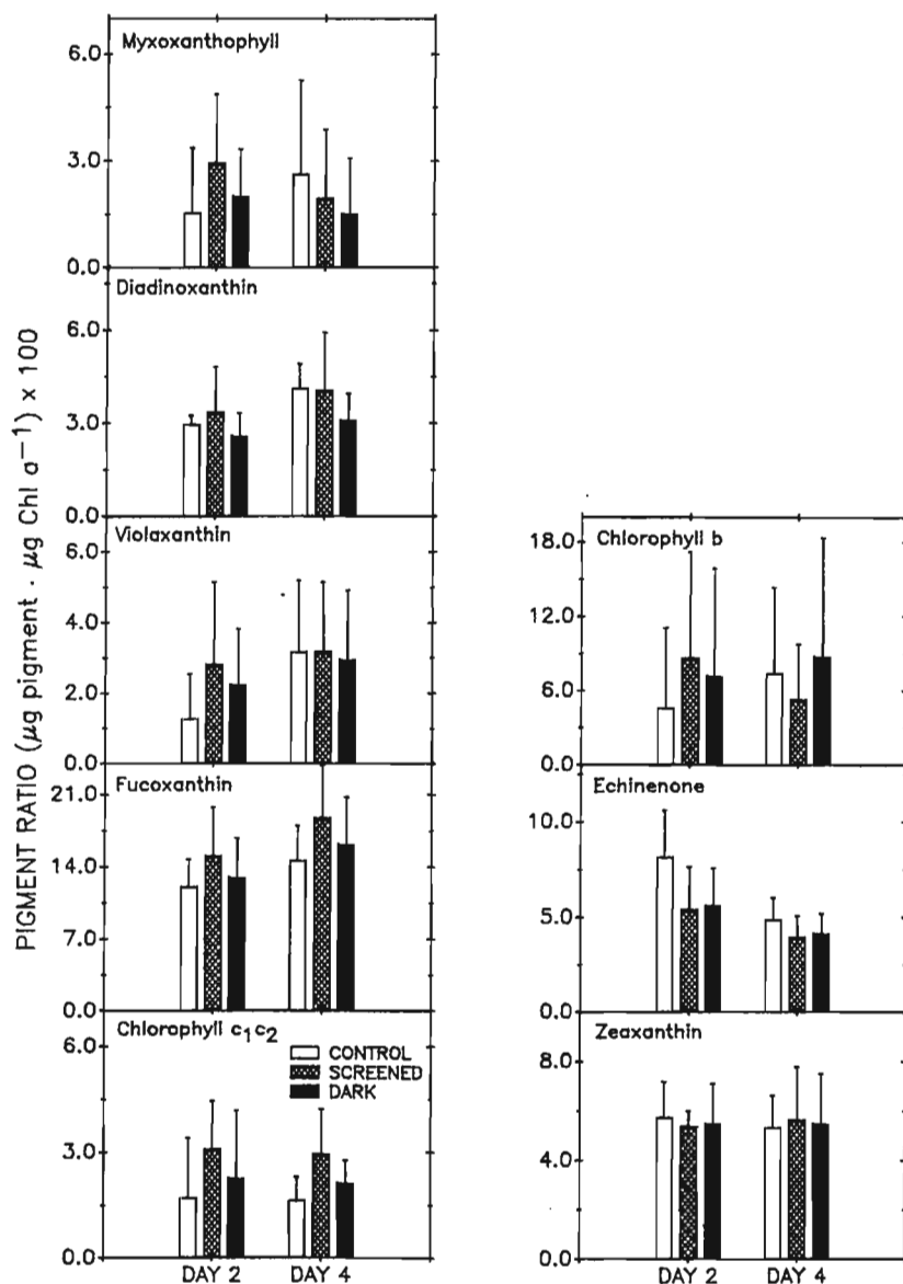
Fig. 7. Results of the photoacclimation experiment showing changes in the ratio of each photopigment to Chl a in three treatments (control, screened, dark) after 2 and 4 days. Values are the mean \pm 1 SD.
