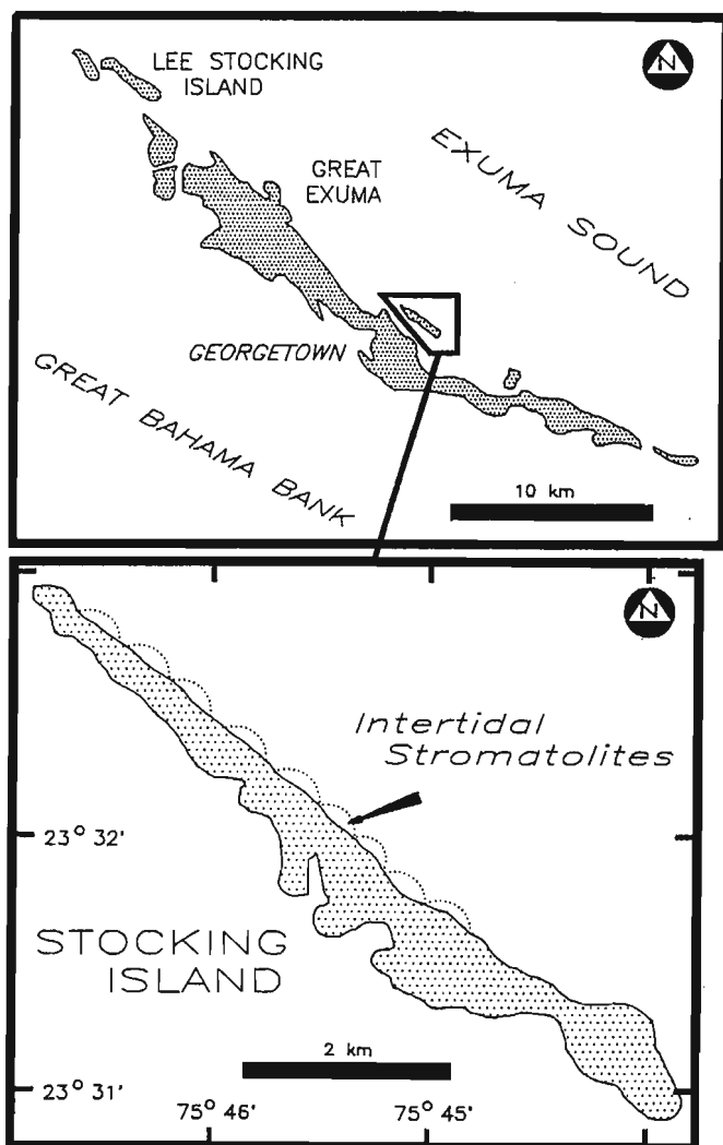
Fig. 1. Maps showing the location of the intertidal stromatolites on Stocking Island, Bahamas. Arrow indicates the location of the study site and horizontal transect (Fig. 2).
