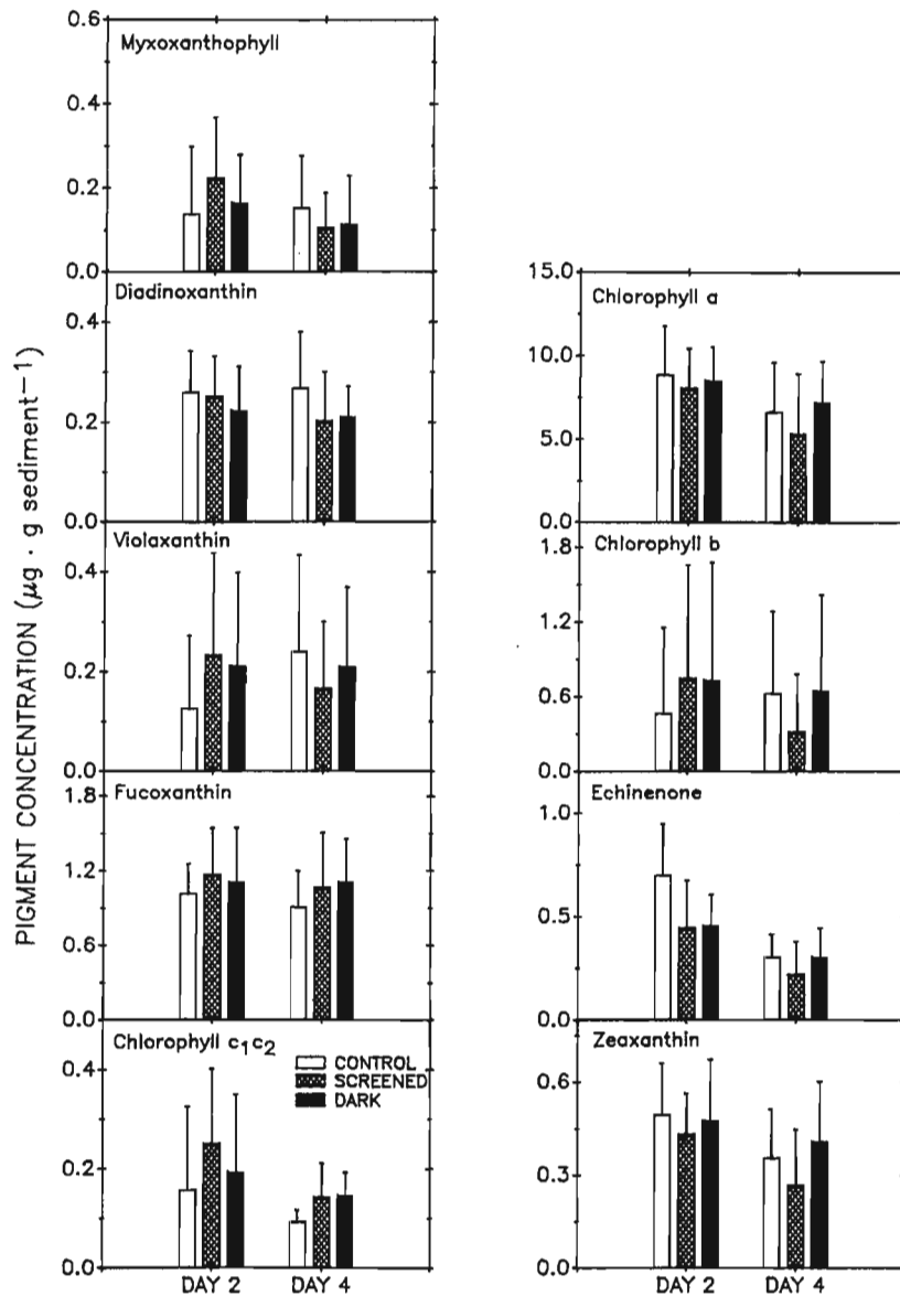
Fig. 6. Results of the photoacclimation experiment showing changes in photopigment concentrations in the three treatments (control, screened, dark) after 2 and 4 days. Values are the mean \pm 1 SD.
